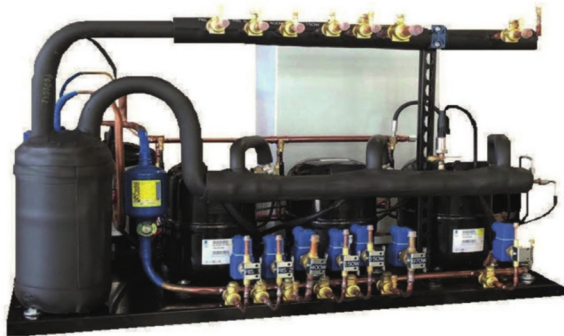
Standard Inverter: LEOCAR-2xCES.4Y
